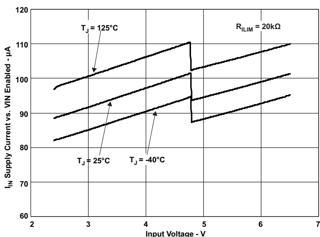
Figure 13. I IN – Supply Current, Output Enabled – μA
