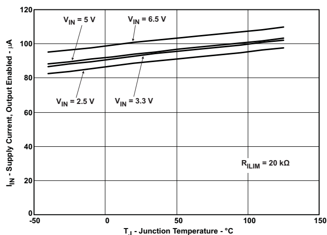
Figure 12. I IN – Supply Current, Output Enabled – μA
